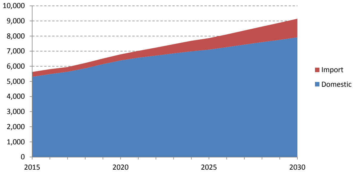
Domestic vs Imported biomass (PJ), HC scenario
