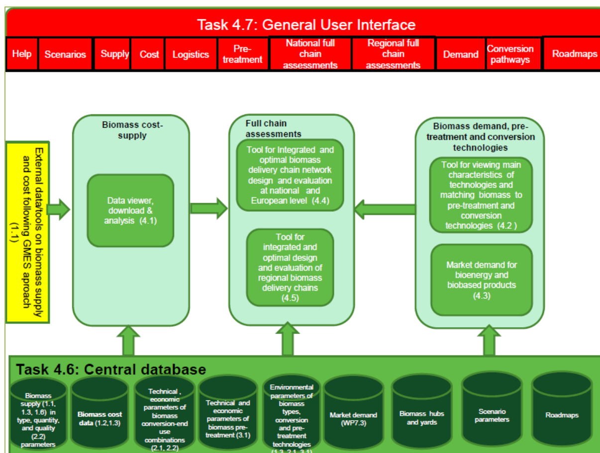
Figure 1: S2Biom General User Interface
